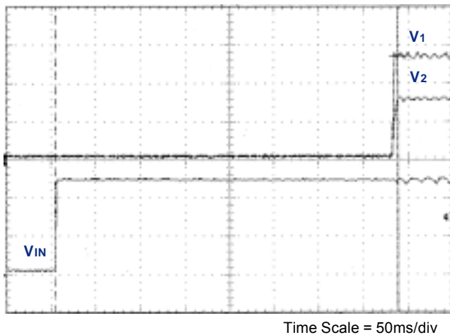
Turn On Time (V IN to V OUT )
