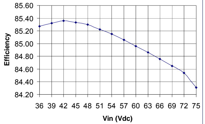
Efficiency vs. Input Voltage @ T_A = +25^\circ\text{C}
