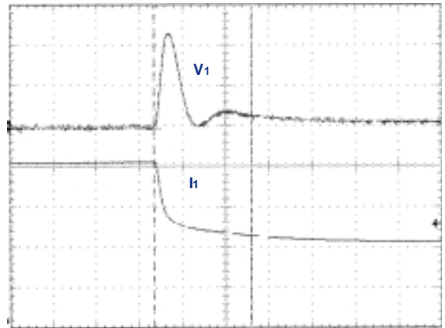
CH1 (1.8Vdc) Transient Response 100% to 50% Load Step
