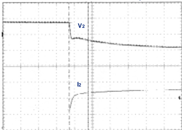
CH2 (1.5Vdc) Transient Response 50% to 100% Load Step
