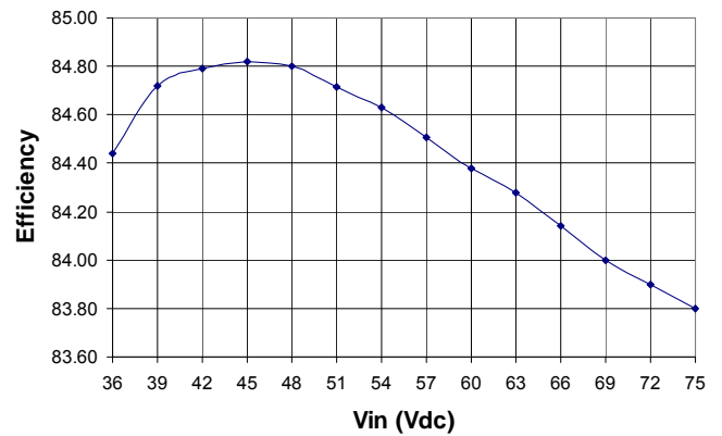
Efficiency vs. Input Voltage @ T_A = +25^\circ\text{C}
