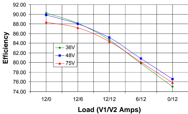
Efficiency vs. Output Current @ T_A = +25^\circ\text{C}
