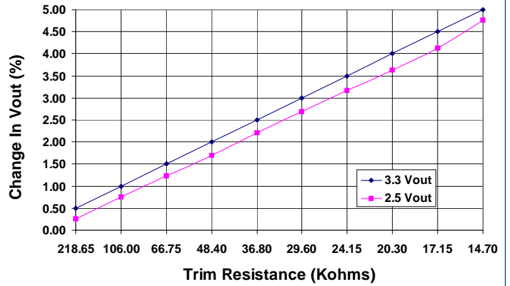
Trim Down Graph
