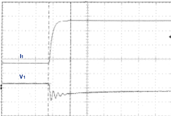
CH1 (5.0Vdc) Transient Response 50% to 100% Load Step
