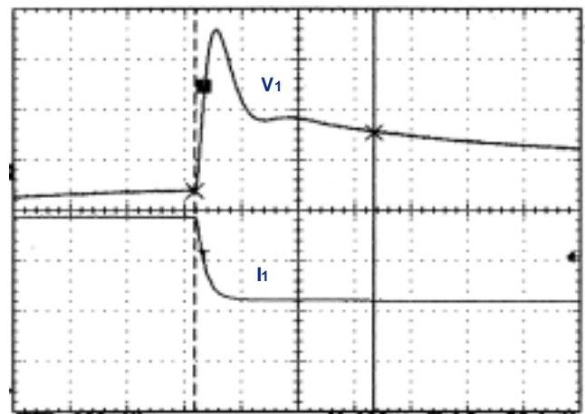
CH1 (3.3Vdc) Transient Response 100% to 50% Load Step
