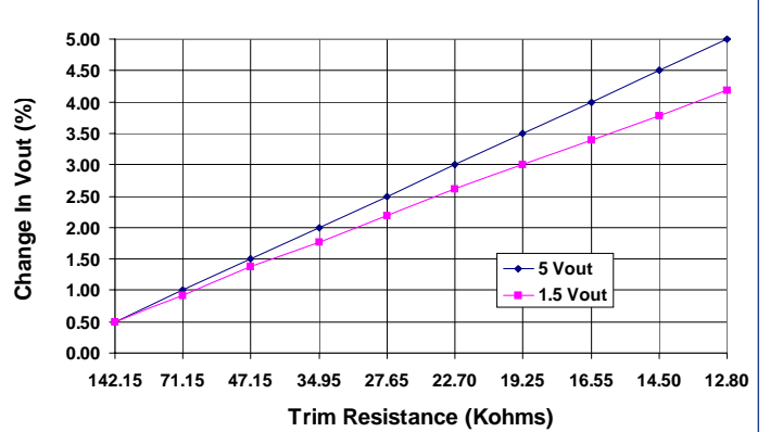
Trim Down Graph
